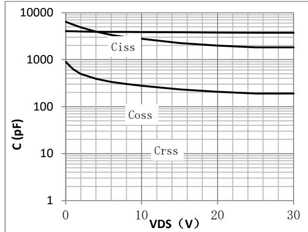
Fig.2 Capacitance Characteristics
