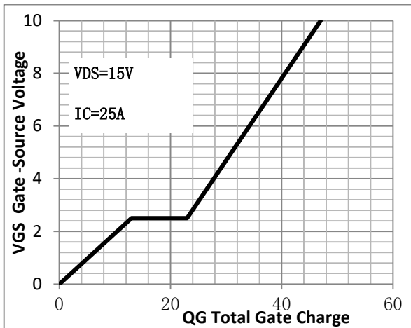
Fig.1 Gate-Charge Characteristics
